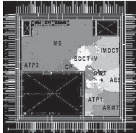
An example of an IC floorplan
